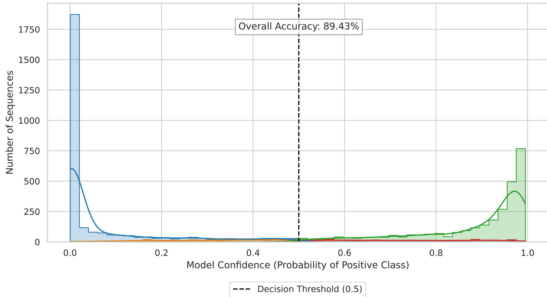
Prediction Confidence Distribution - HMB-Net (Atlas_r_m6A)
