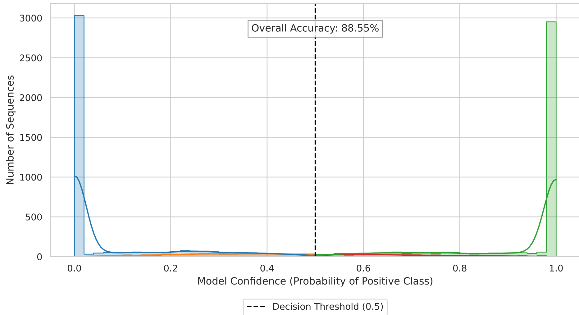
Prediction Confidence Distribution - HMB-Net (RMBase_h_m6A)
