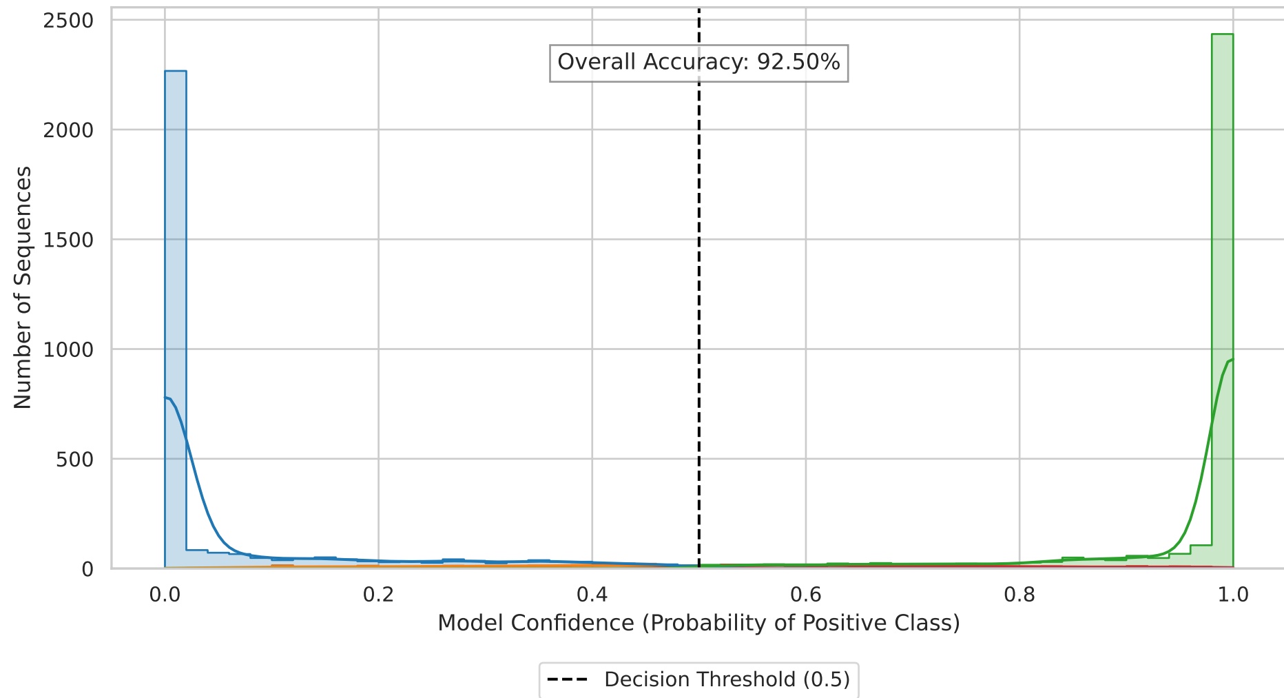
Prediction Confidence Distribution - HMB-Net (RMBase_r_m6A)
