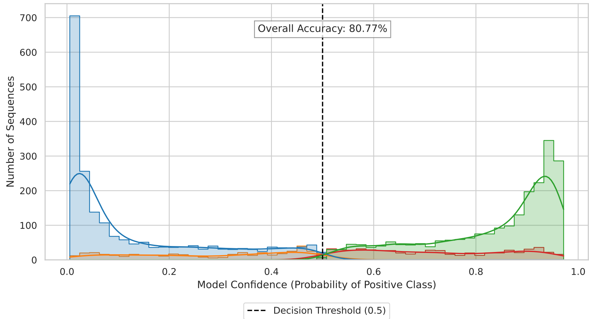
Prediction Confidence Distribution - HMB-Net (h_I)
