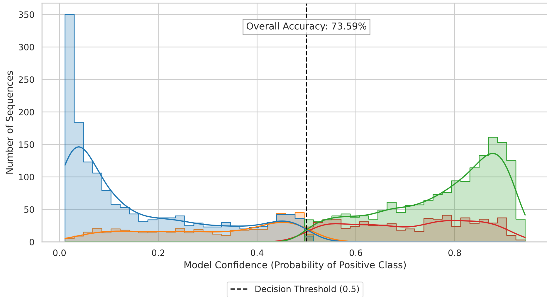
Prediction Confidence Distribution - HMB-Net (m_h)
