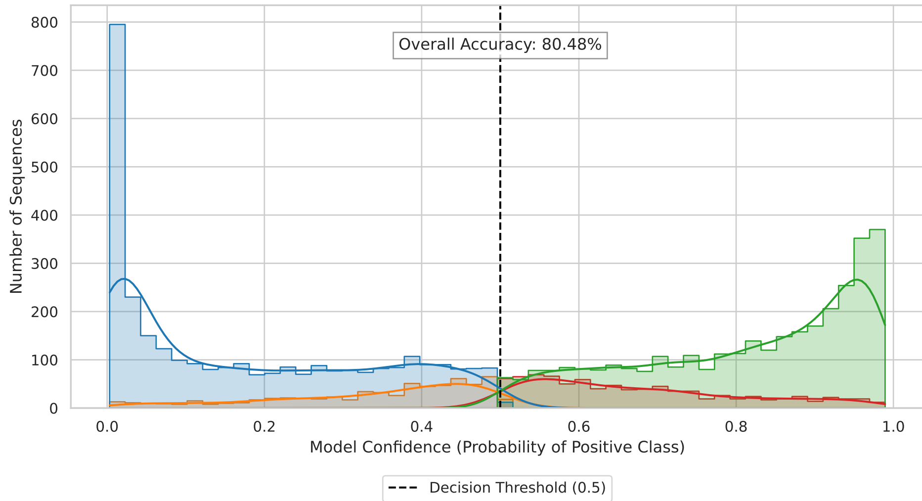
Prediction Confidence Distribution - HMB-Net (m_k)
