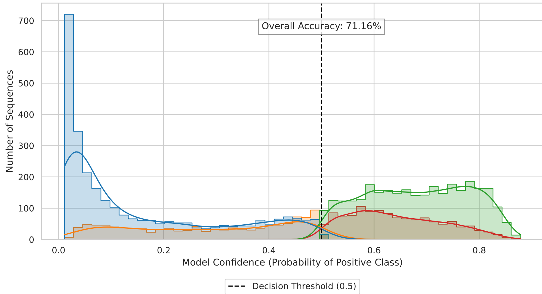
Prediction Confidence Distribution - HMB-Net (m_l)
