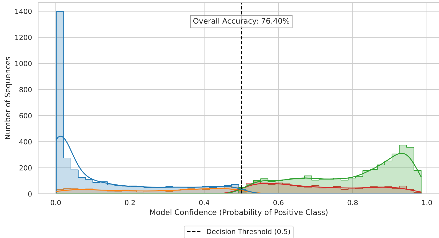
Prediction Confidence Distribution - HMB-Net (m_t)
