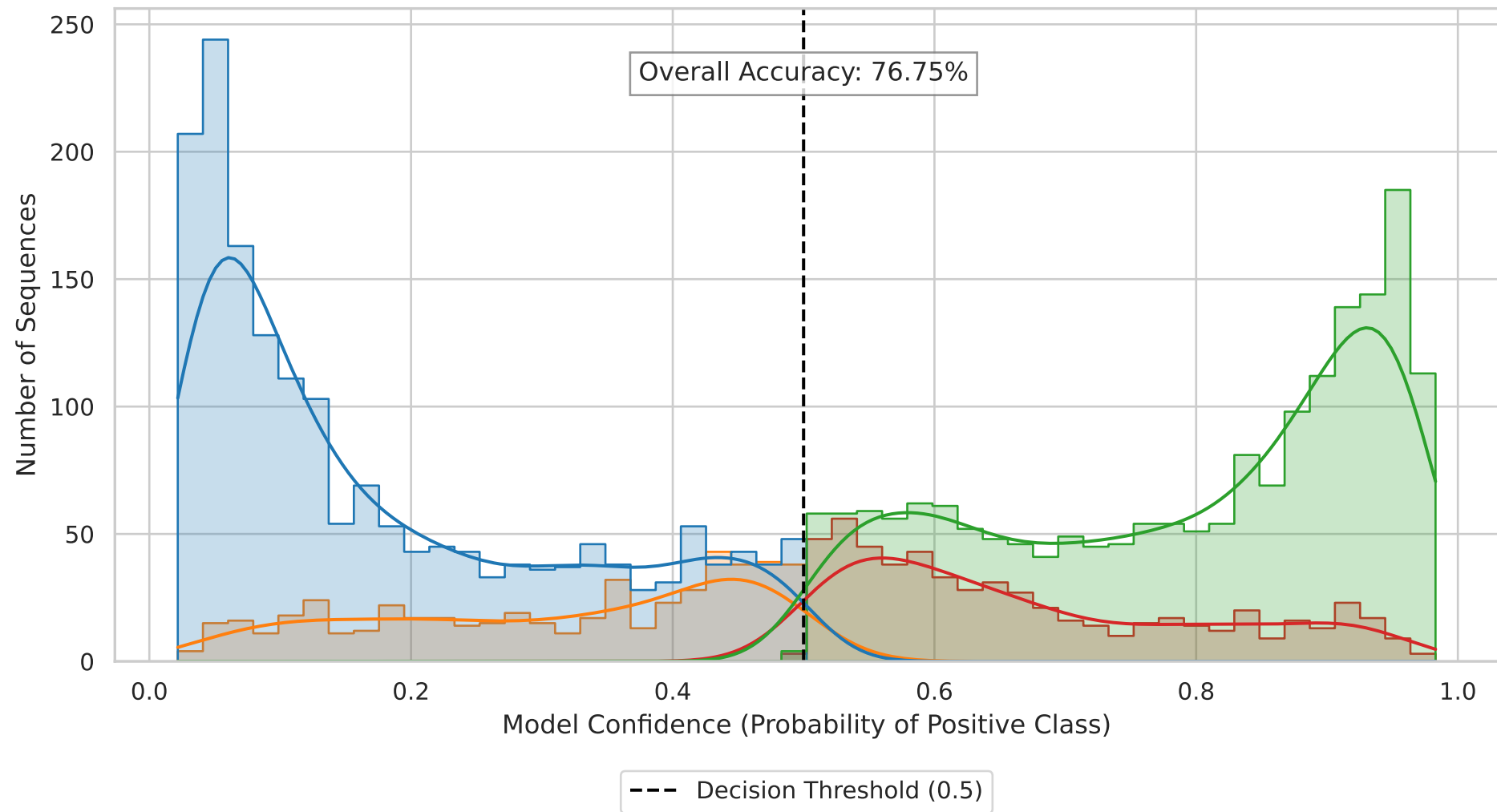
Prediction Confidence Distribution - HMB-Net (r_b)
