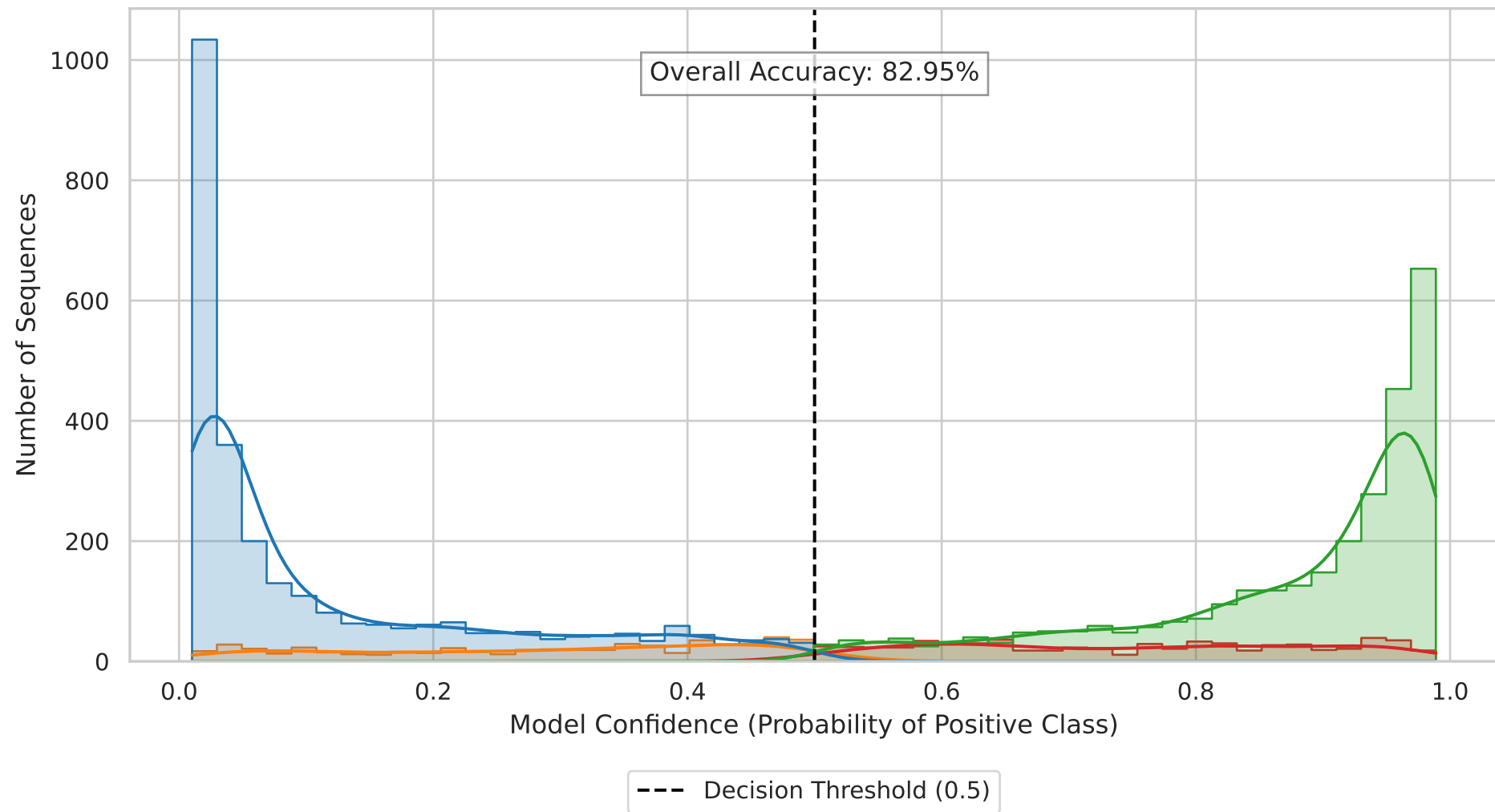
Prediction Confidence Distribution - HMB-Net (r_k)
