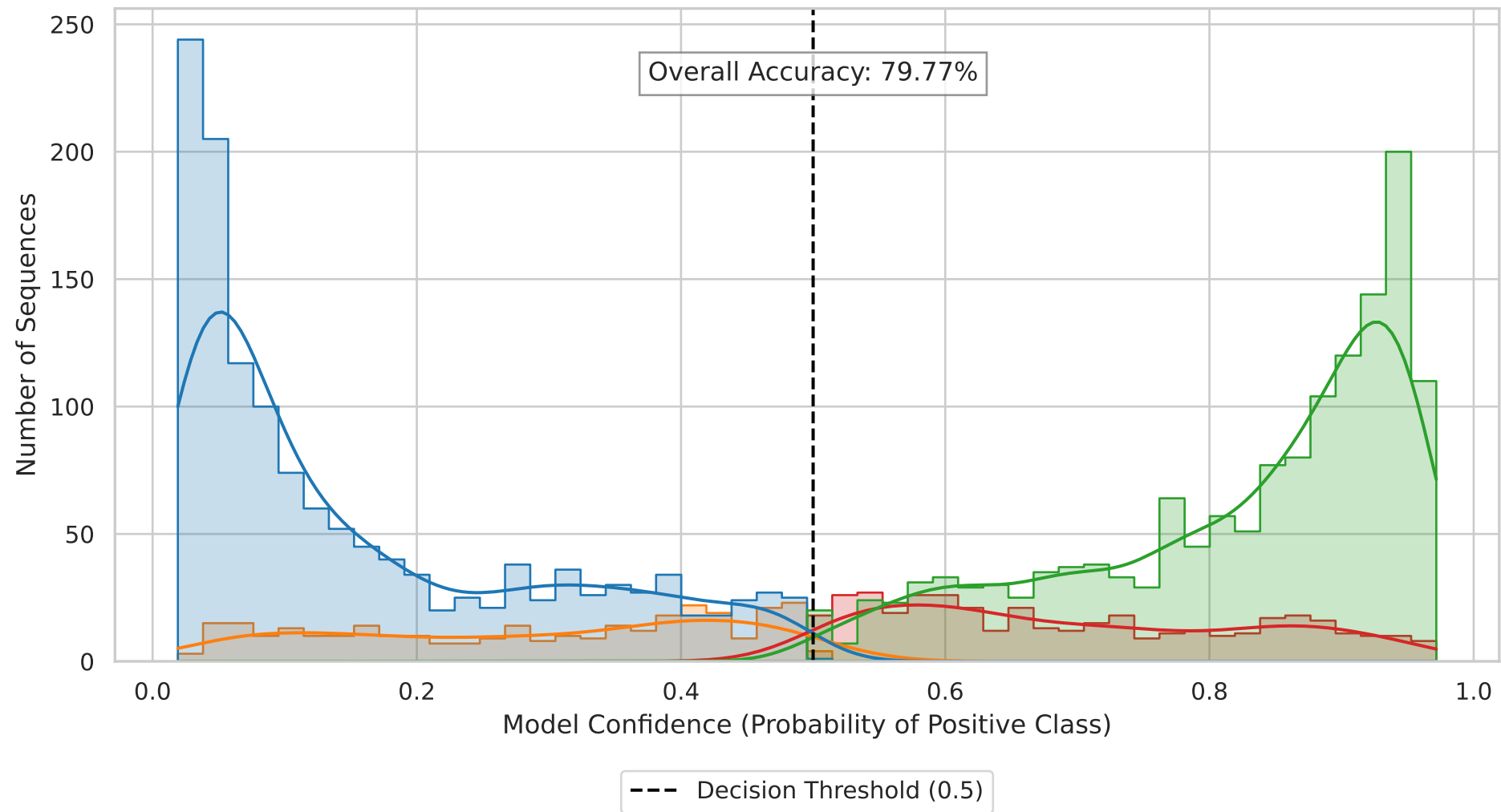
Prediction Confidence Distribution - HMB-Net (r_l)
