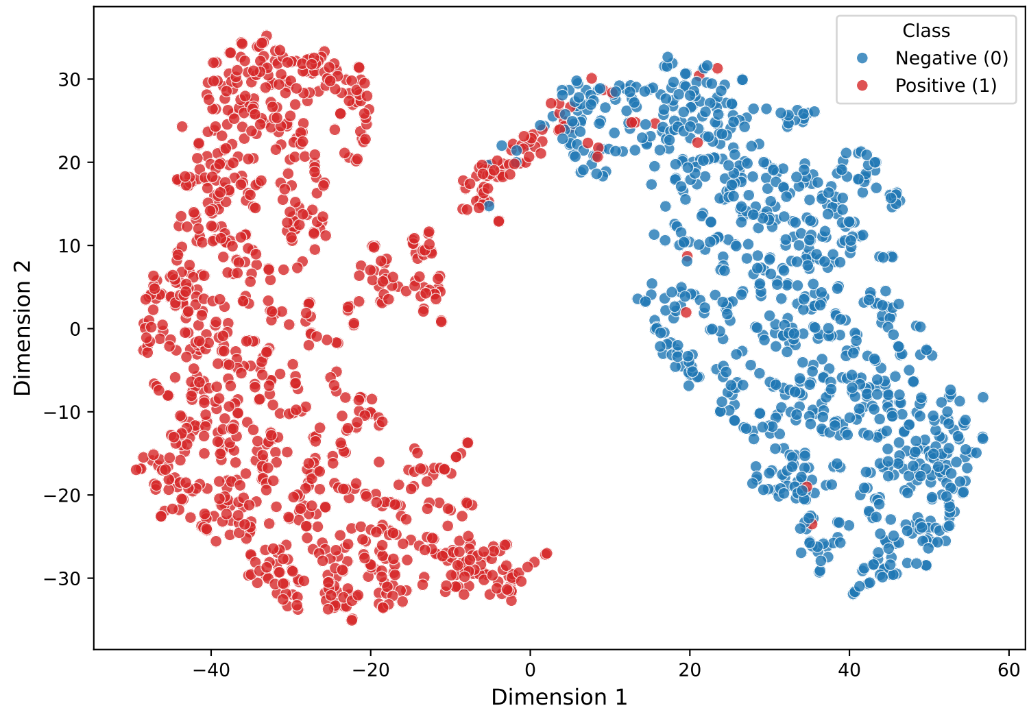
t-SNE of HMB-Net (Atlas_h_m1A)
