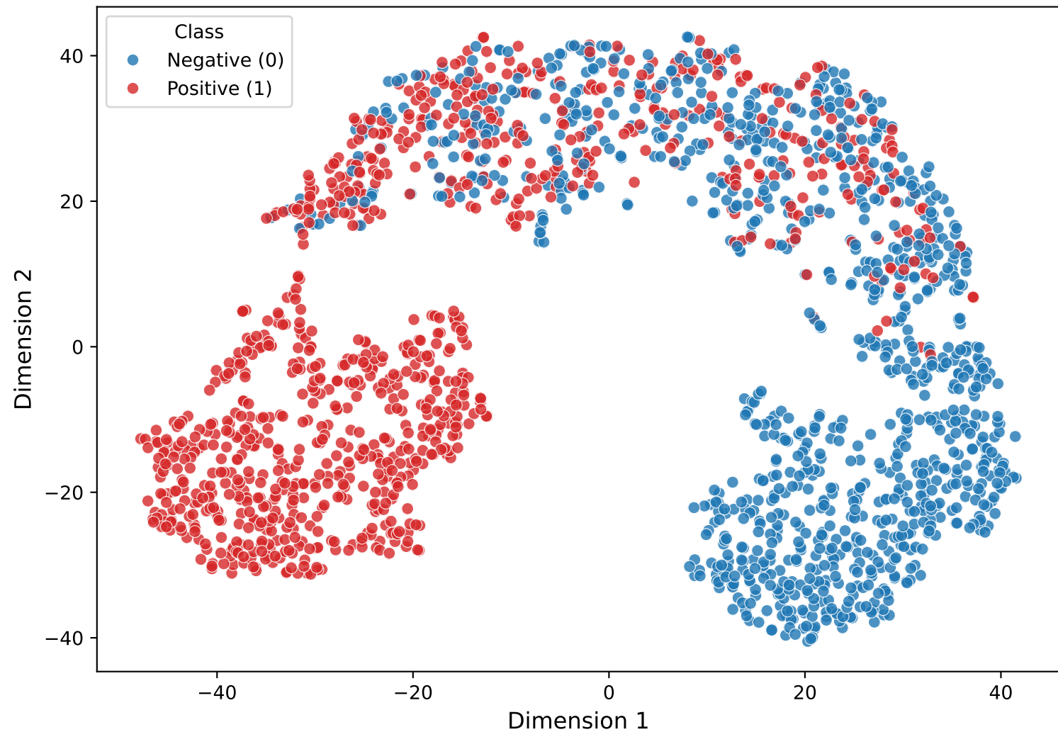
t-SNE of HMB-Net (Atlas_m_m1A)
