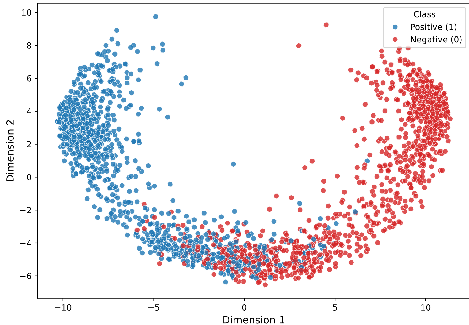
PCA of HMB-Net (Atlas_m_m6A)
