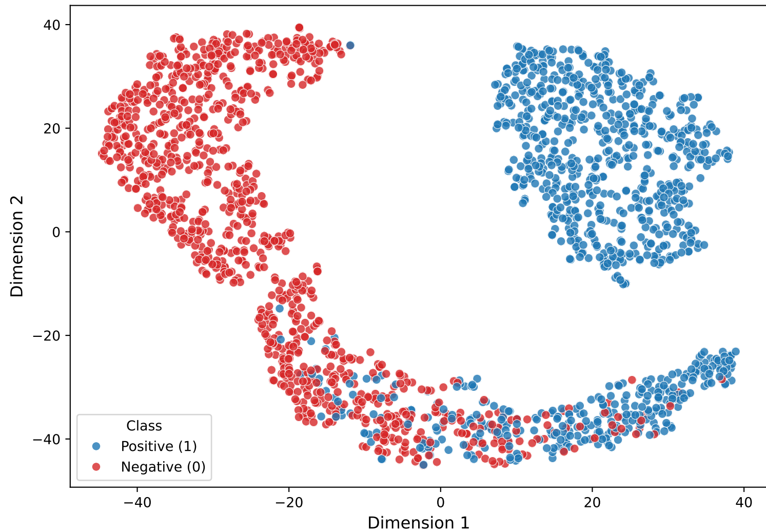
t-SNE of HMB-Net (RMBase_r_m6A)
