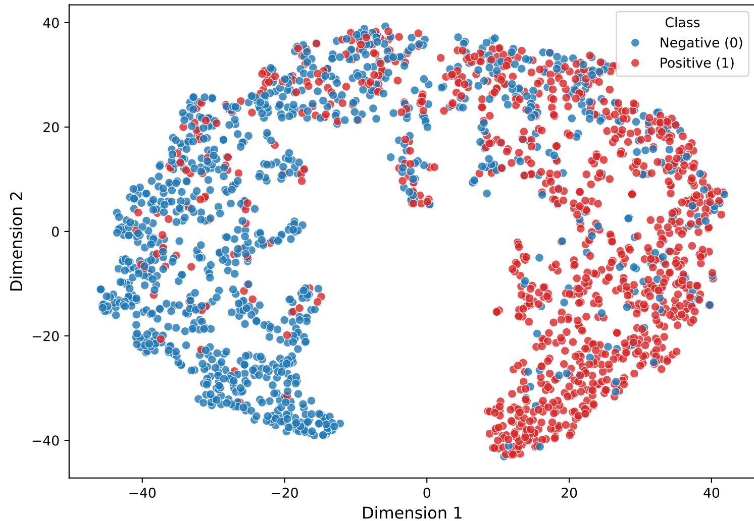
t-SNE of HMB-Net (h_l)
