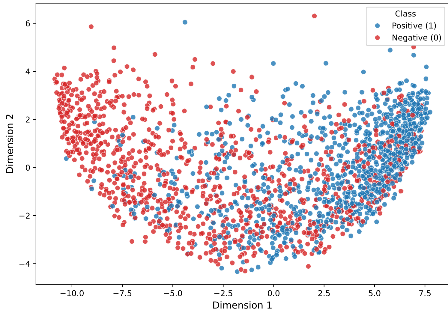
PCA of HMB-Net (m_h)
