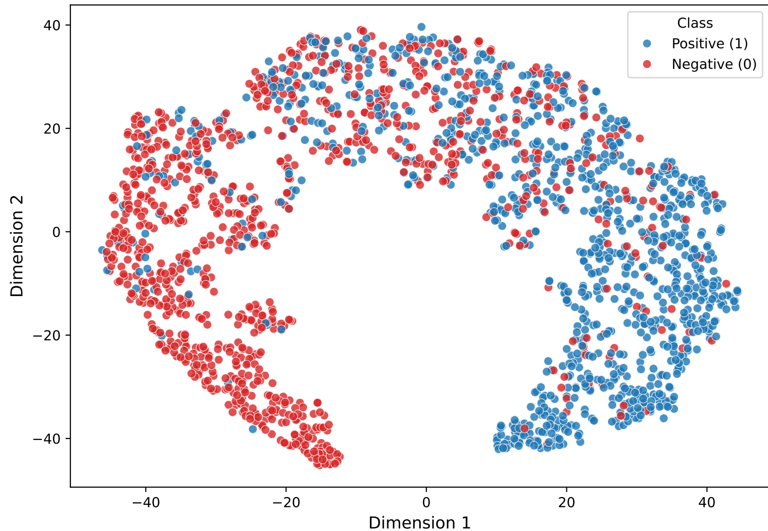
t-SNE of HMB-Net (m_k)
