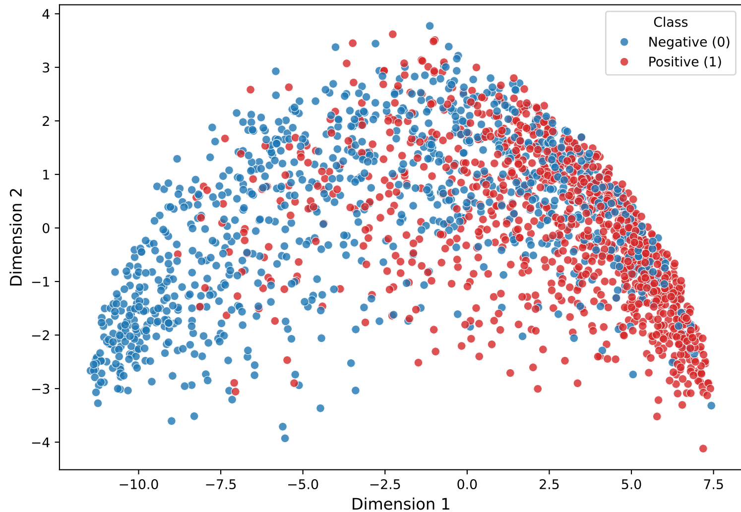
PCA of HMB-Net (m_l)
