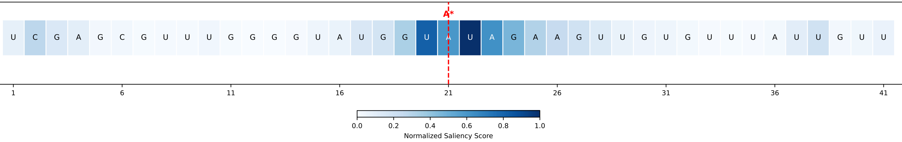
Sample #1323 | Confidence: 0.9650 | DRACH motifs found: 0 | Seq: UCGAGCGUUUGG...
