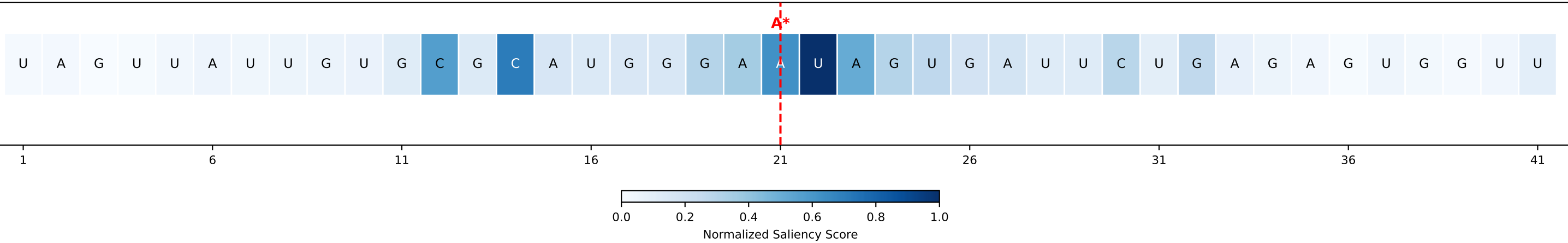
Sample #1913 | Confidence: 0.9408 | DRACH motifs found: 0 | Seq: UAGUUAUUGUGC...
