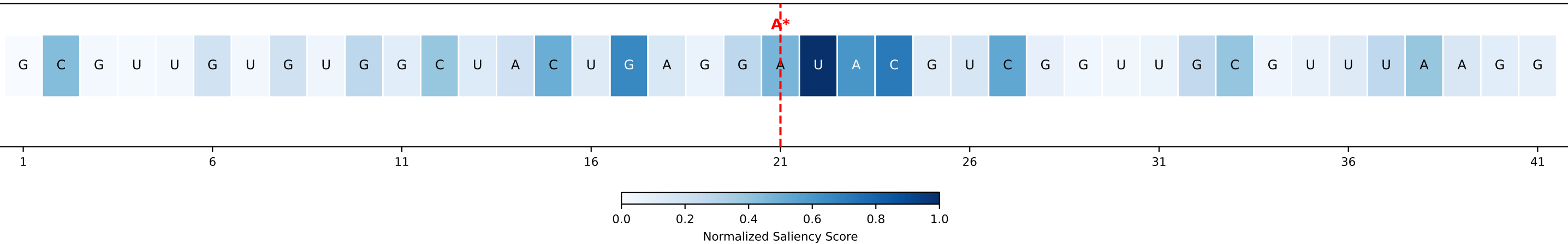
Sample #807 | Confidence: 0.9394 | DRACH motifs found: 0 | Seq: GCGUUGUGUGGC...
