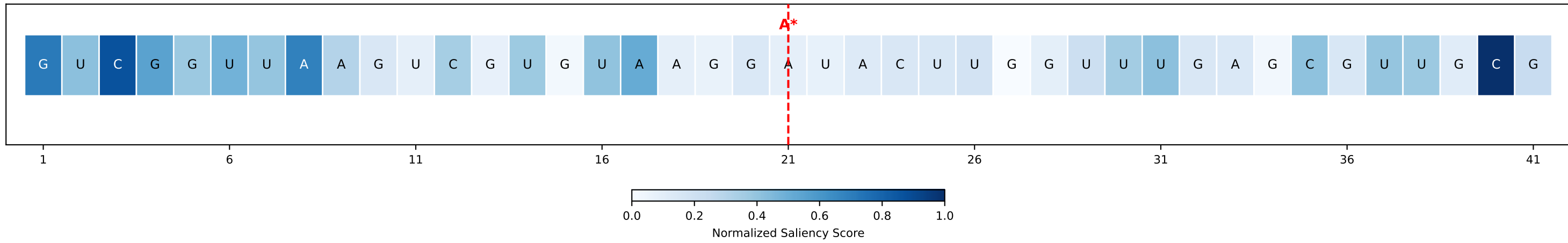
Sample #3760 | Confidence: 0.9813 | DRACH motifs found: 0 | Seq: GUCGGUUAAGUC...
