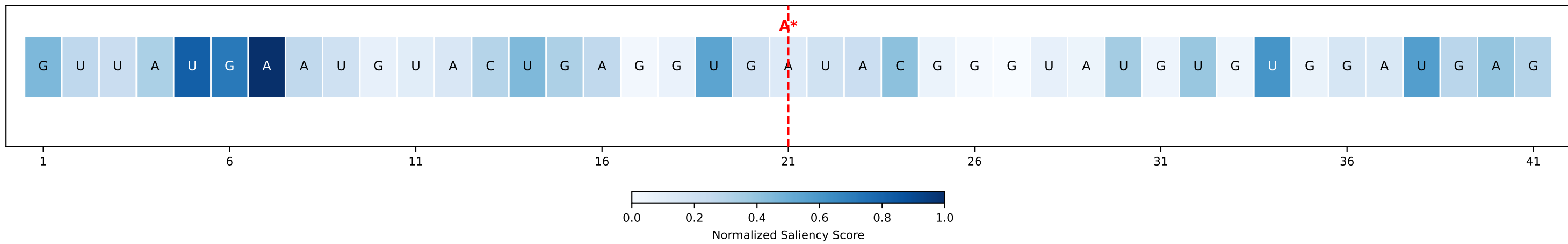
Sample #4629 | Confidence: 0.9831 | DRACH motifs found: 0 | Seq: GUUAUGAAUGUA...
