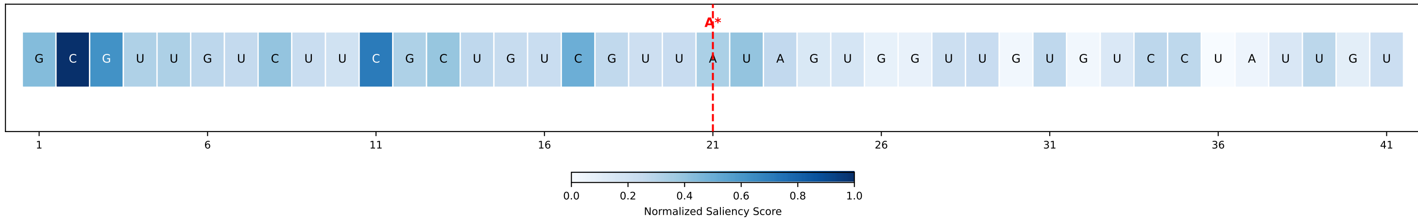
Sample #3613 | Confidence: 0.9825 | DRACH motifs found: 0 | Seq: GCGUUGUCUUCG...
