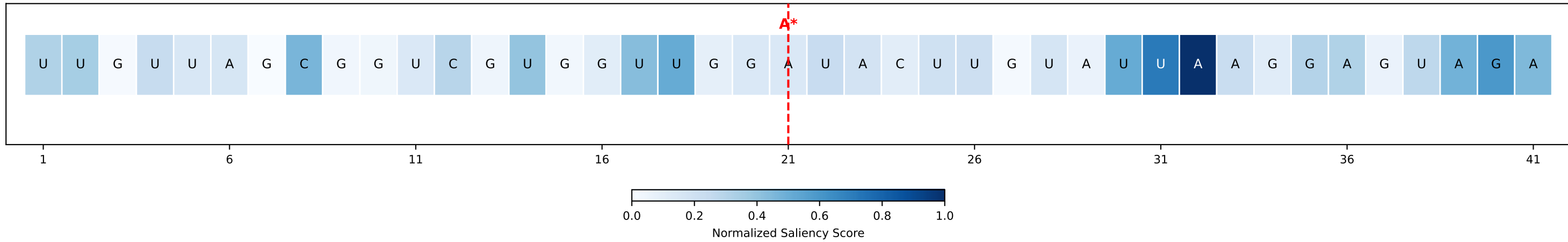
Sample #2300 | Confidence: 0.9822 | DRACH motifs found: 0 | Seq: UUGUUAGCGGUC...
