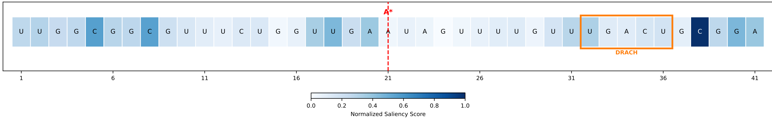
Sample #1633 | Confidence: 0.9827 | DRACH motifs found: 1 | Seq: UUGGCGGCGUUU...
