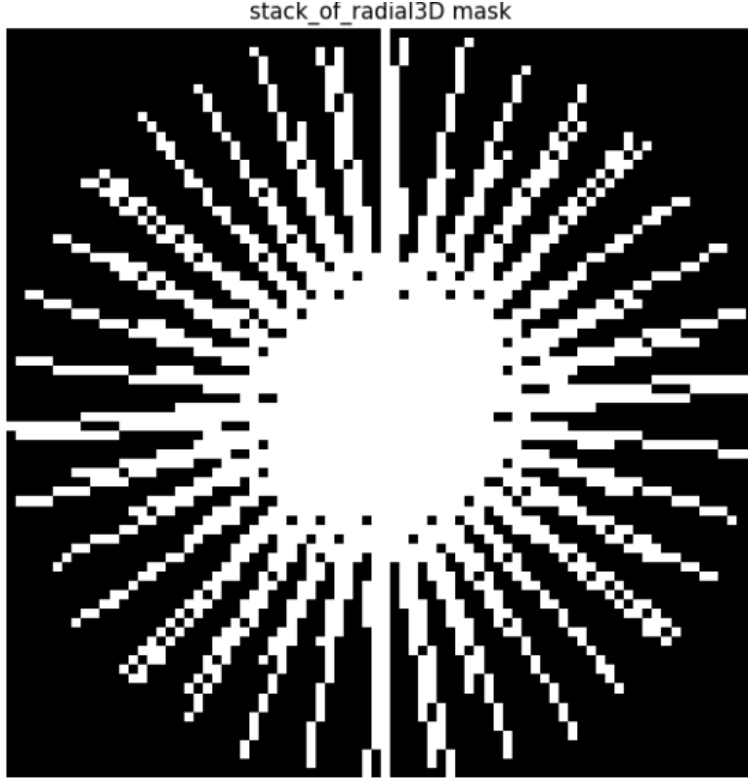
Figure 7: Representation of a slice of a 3D radial mask
