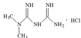
Cloridrato de metformina
