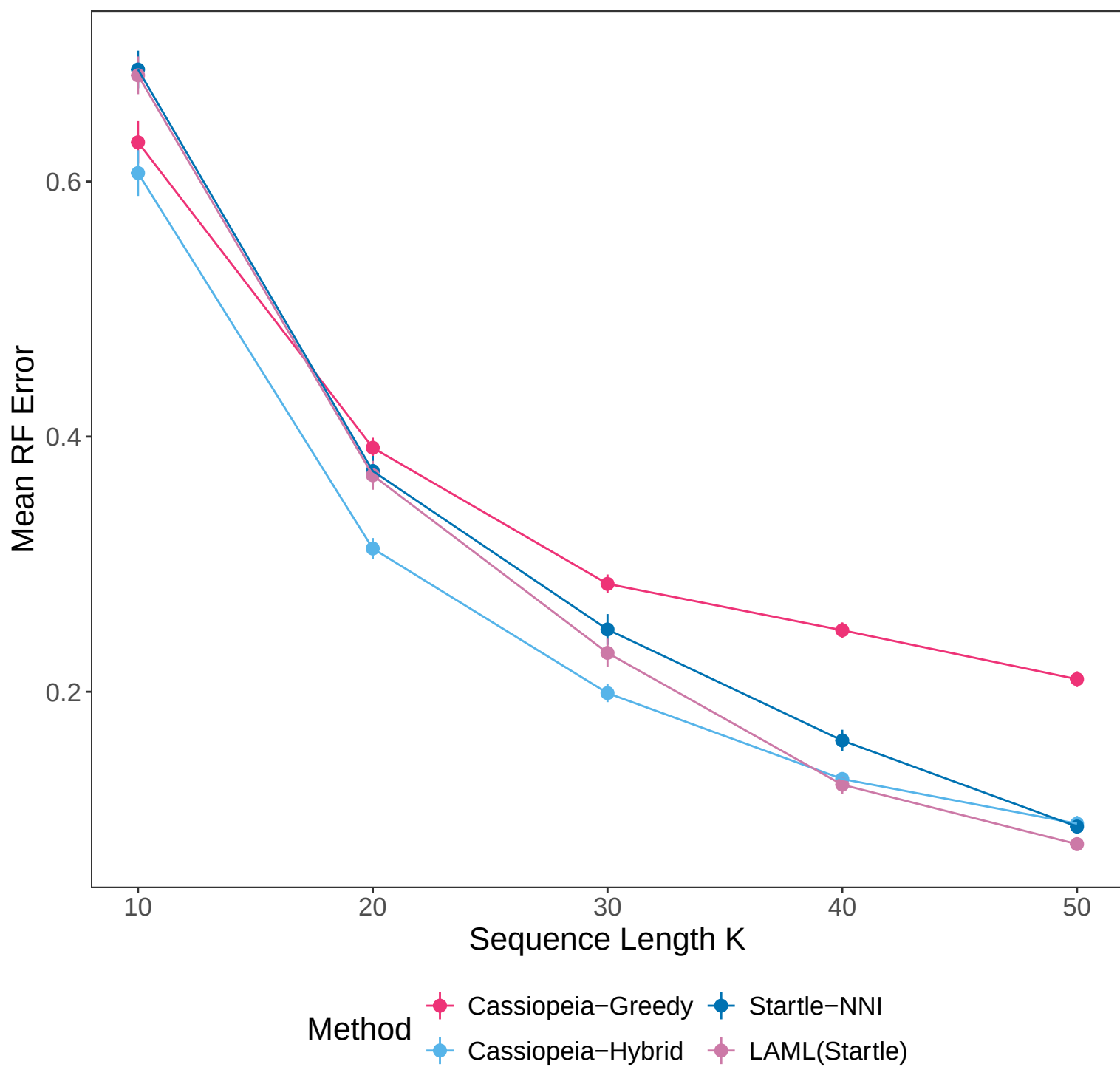
RF Error Over Sequence Length K (s0d0)
