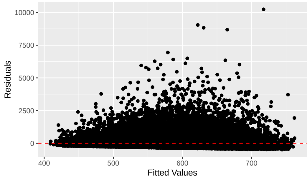
Residuals vs Fitted for baseline factors
