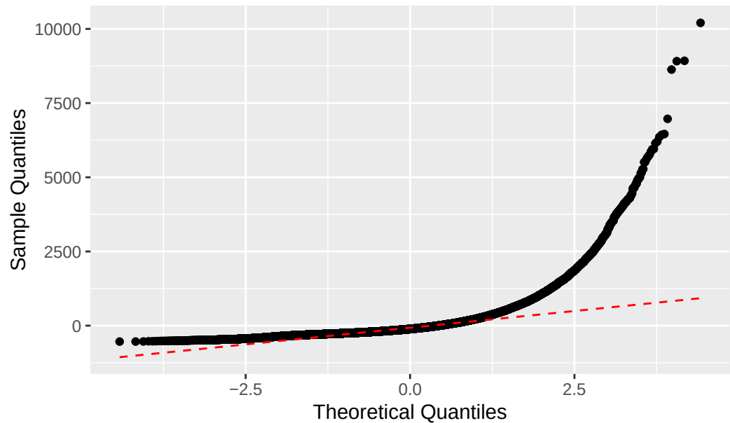
Q-Q Plot for baseline factors
