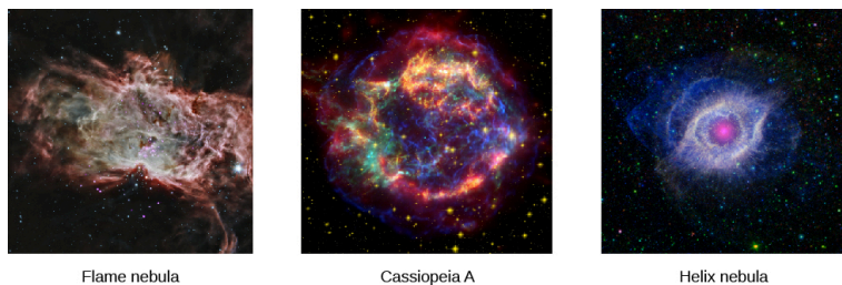
Figure 2. These infrared images—a region of star formation, the remnant of an exploded star, and a region where an old star is
