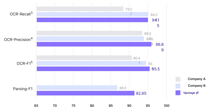
Upstage universal OCR model performance details: Document criteria
