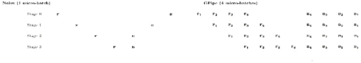
Figure 11.7: Pipeline bubble comparison. Left: naive pipeline with one micro-batch has 75% idle time. Right: GPipe with M = 4 micro-batches reduces bubbles significantly. With M \gg P , bubble fraction approaches zero.
