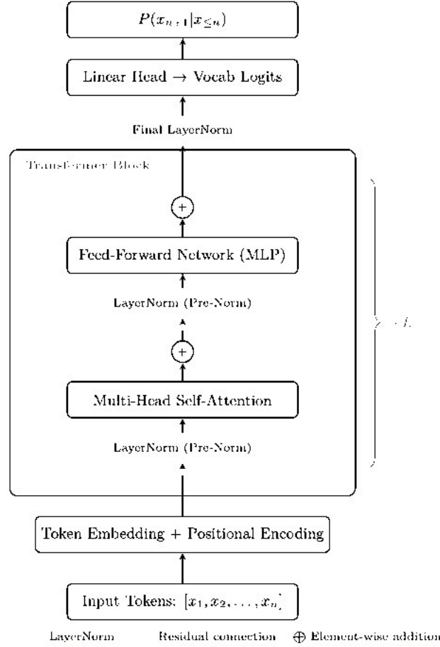
Figure 1.3: Decoder-only Transformer block (GPT-style, Pre-Norm variant). Each sub-layer (attention, FFN) is preceded by LayerNorm and followed by a residual addition: \mathbf{x} + \text{SubLayer}(\text{LN}(\mathbf{x})) . This Pre-Norm ordering (used by Llama, GPT-3, Mistral) stabilizes training without warmup, unlike the original Post-Norm (which applies LayerNorm after the addition). L identical blocks are stacked, followed by a final LayerNorm and linear projection to vocabulary logits.
