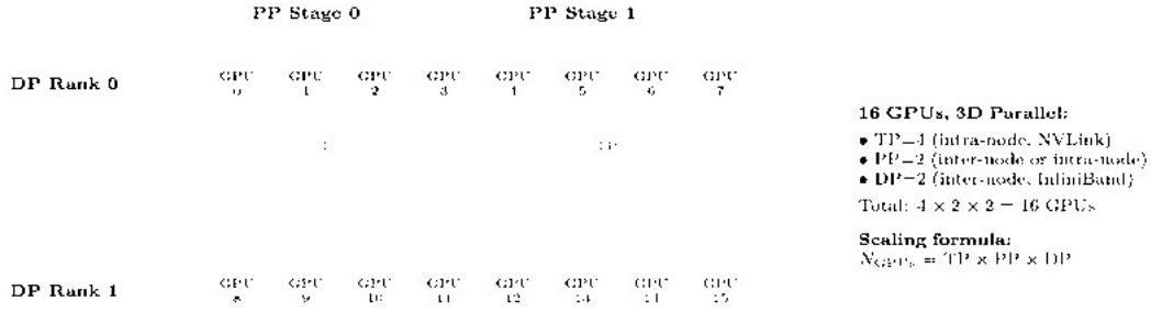
Figure 11.9: 3D parallelism layout for 16 GPUs: TP=4 (within each box, using NVLink), PP=2 (orange arrows, stages), DP=2 (red arrows, gradient sync). Each dimension exploits a different level of the communication hierarchy.
