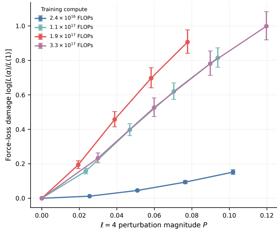
A. High-order features are causally required in trained eSEN
