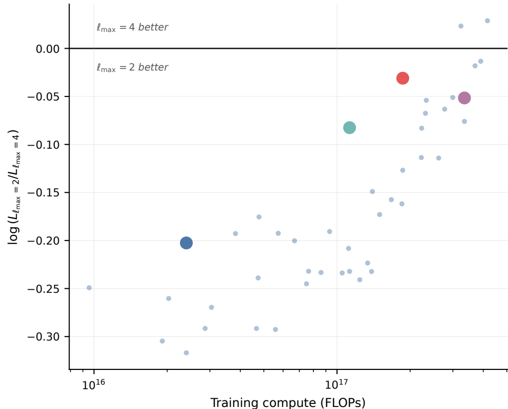
B. Causal use does not imply matched-compute advantage
