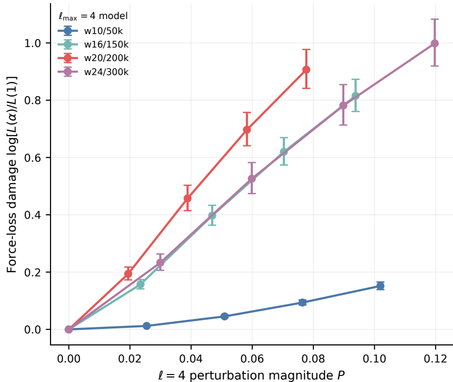
A. High-order features are causally required in trained eSEN
