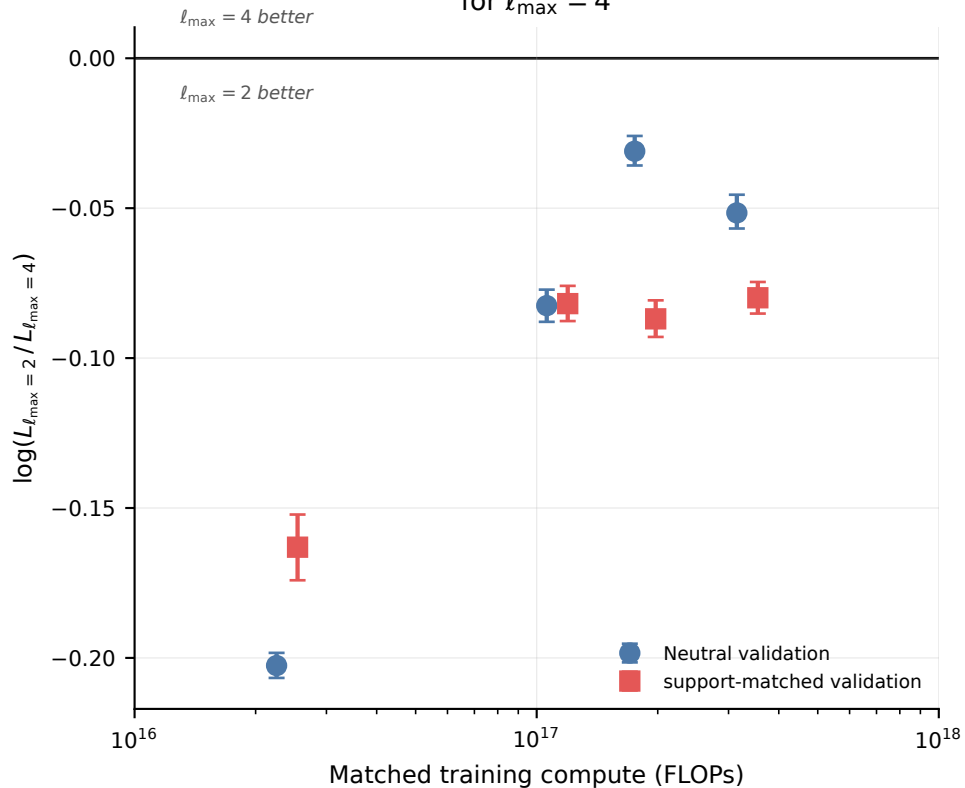
B. No matched-compute advantage for \ell_{\max} = 4
