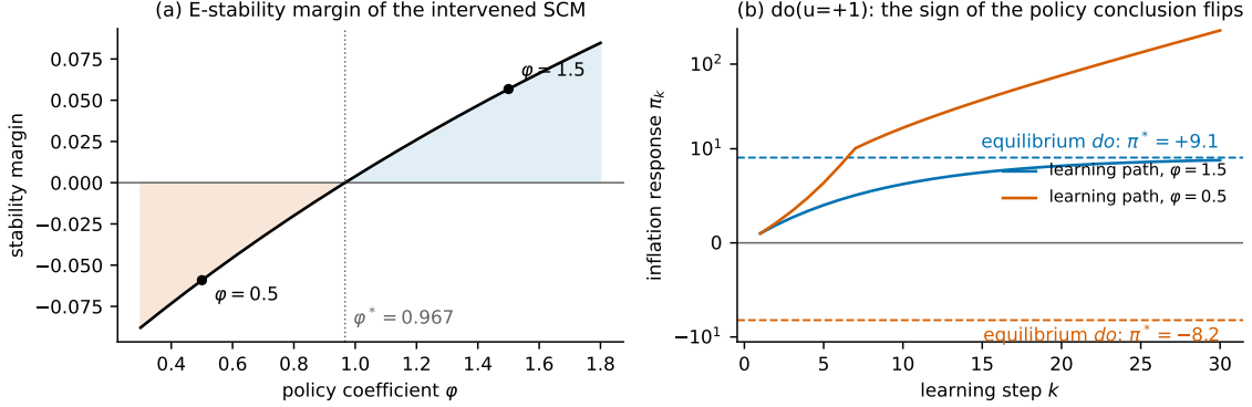
Figure 1: E4. Left: stability margin of the intervened SCM as a function of the policy coefficient \varphi , crossing zero at \varphi^* = 0.9667 . Right: under \text{do}(u=+1) , naive-expectations learning paths against the equilibrium predictions (dashed): at \varphi = 1.5 they agree (IDENTIFIED, gap 7 \times 10^{-15} ); at \varphi = 0.5 the equilibrium predicts \pi^* = -8.21 while learning explodes upward ( \pi_{30} = +249.6 ) — the sign of the policy conclusion flips, and the certificate reports margin = -0.059 with \gamma^* = 0 : no learning rate rescues it.
