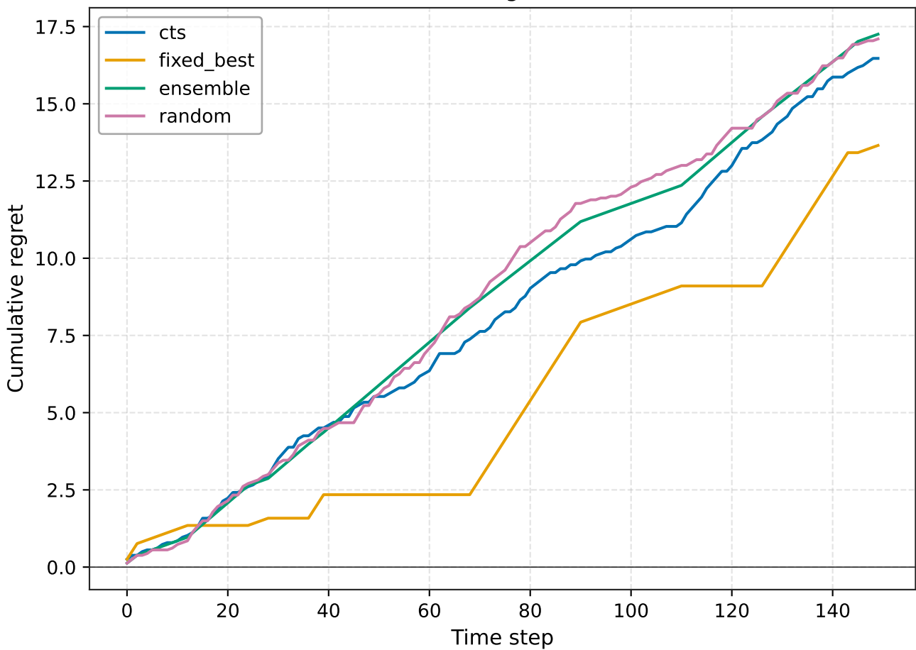
Cumulative Regret vs Oracle
