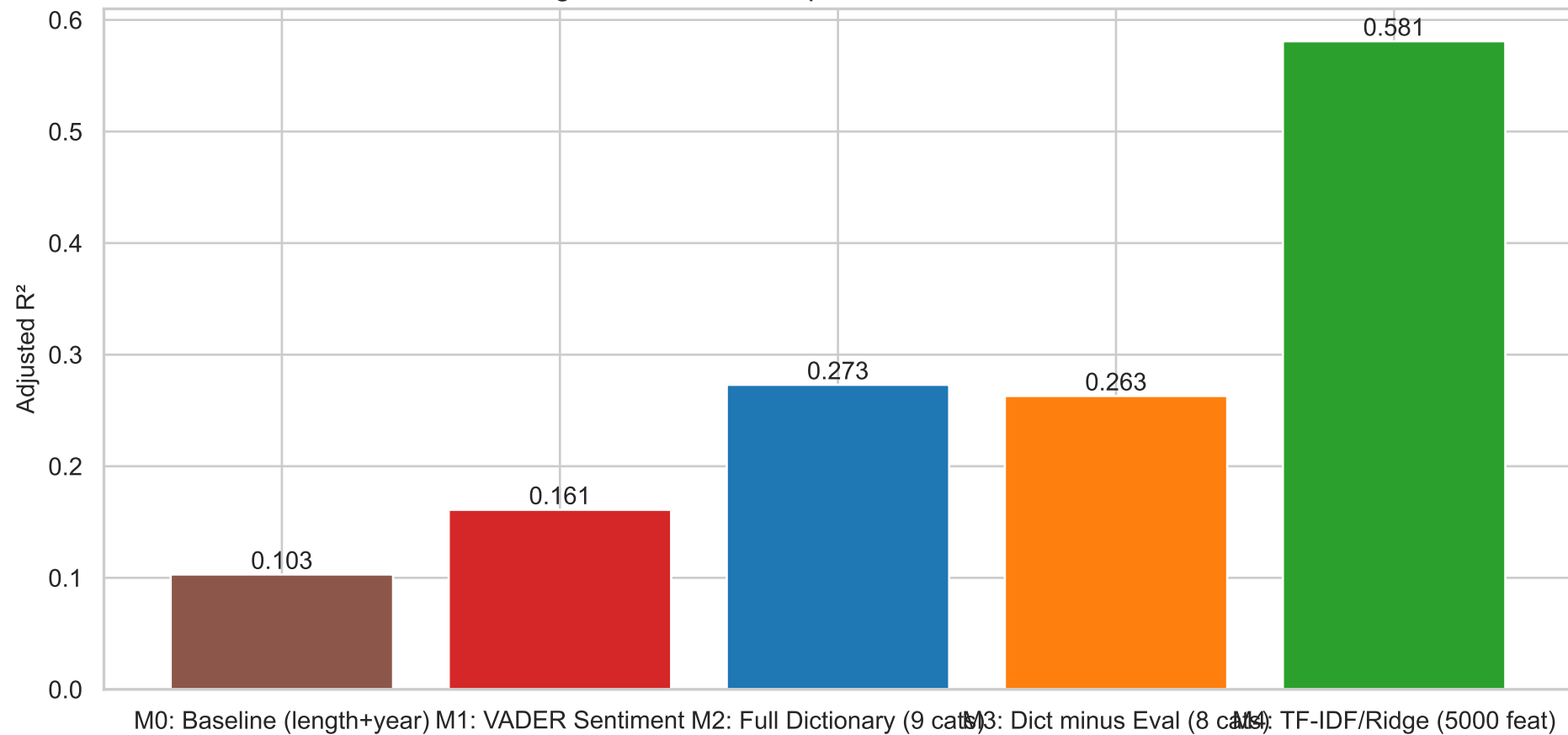
Figure W4-1: R^2 Comparison — All Five Models
