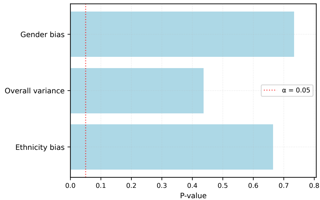
All Permutation Test P-values
