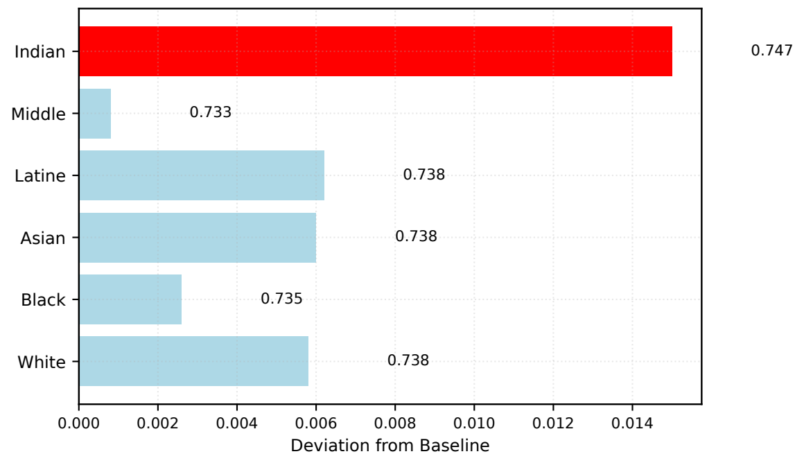
Ethnicity Group Deviations (Baseline: 0.7320)
