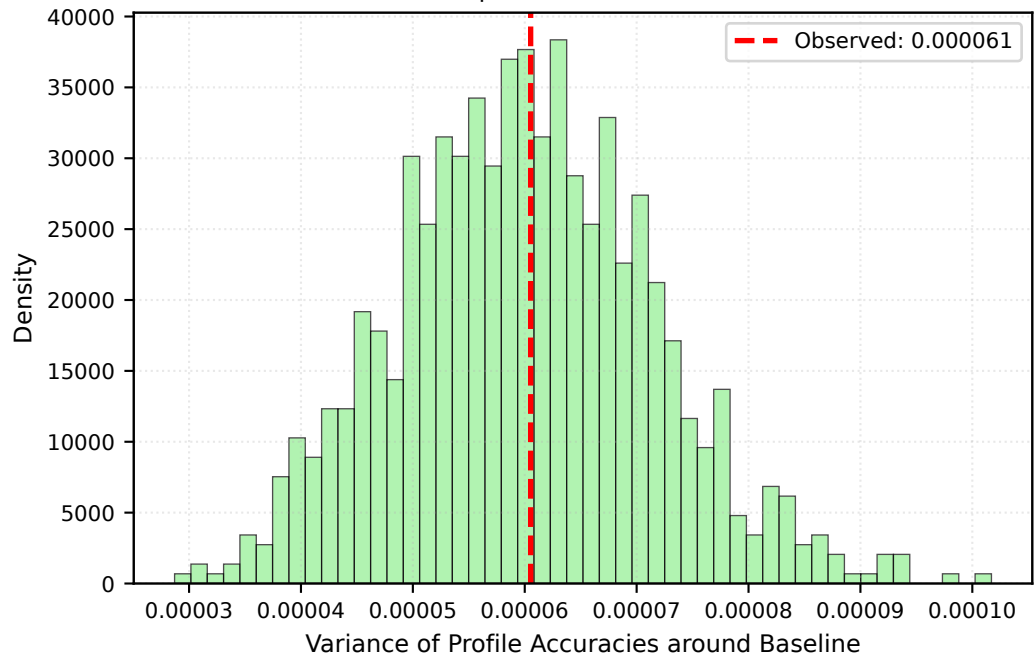
Overall Profile Variance Test p-value = 0.4785
