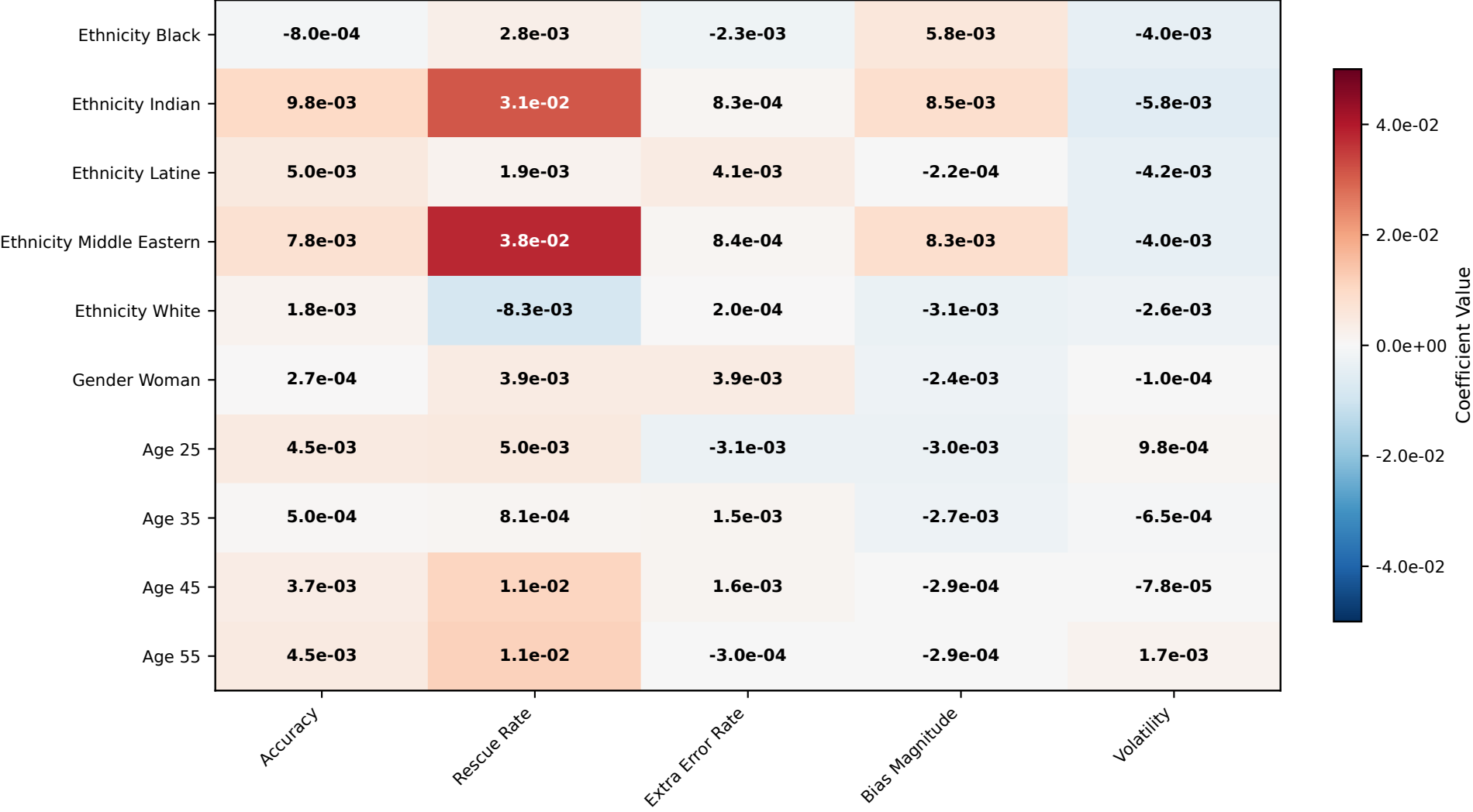
Causal Path Coefficients ( \beta )
