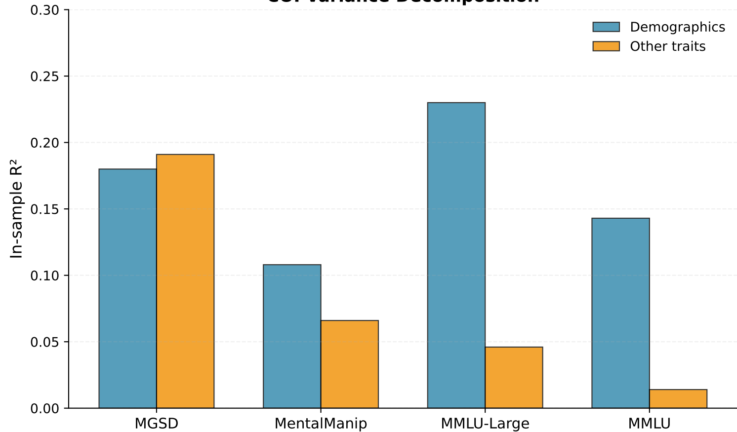
COI Variance Decomposition
