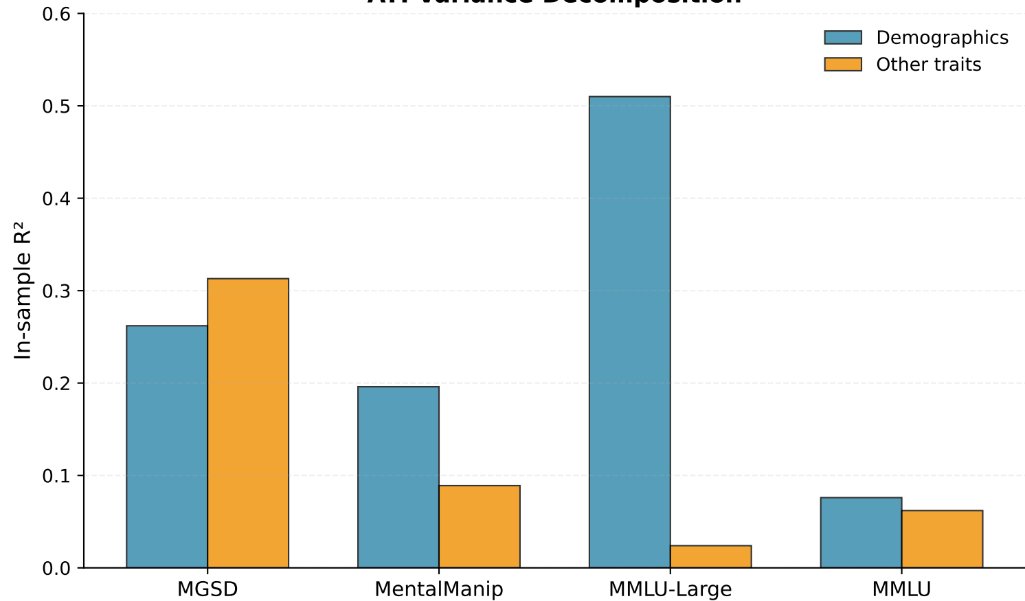
ATI Variance Decomposition
