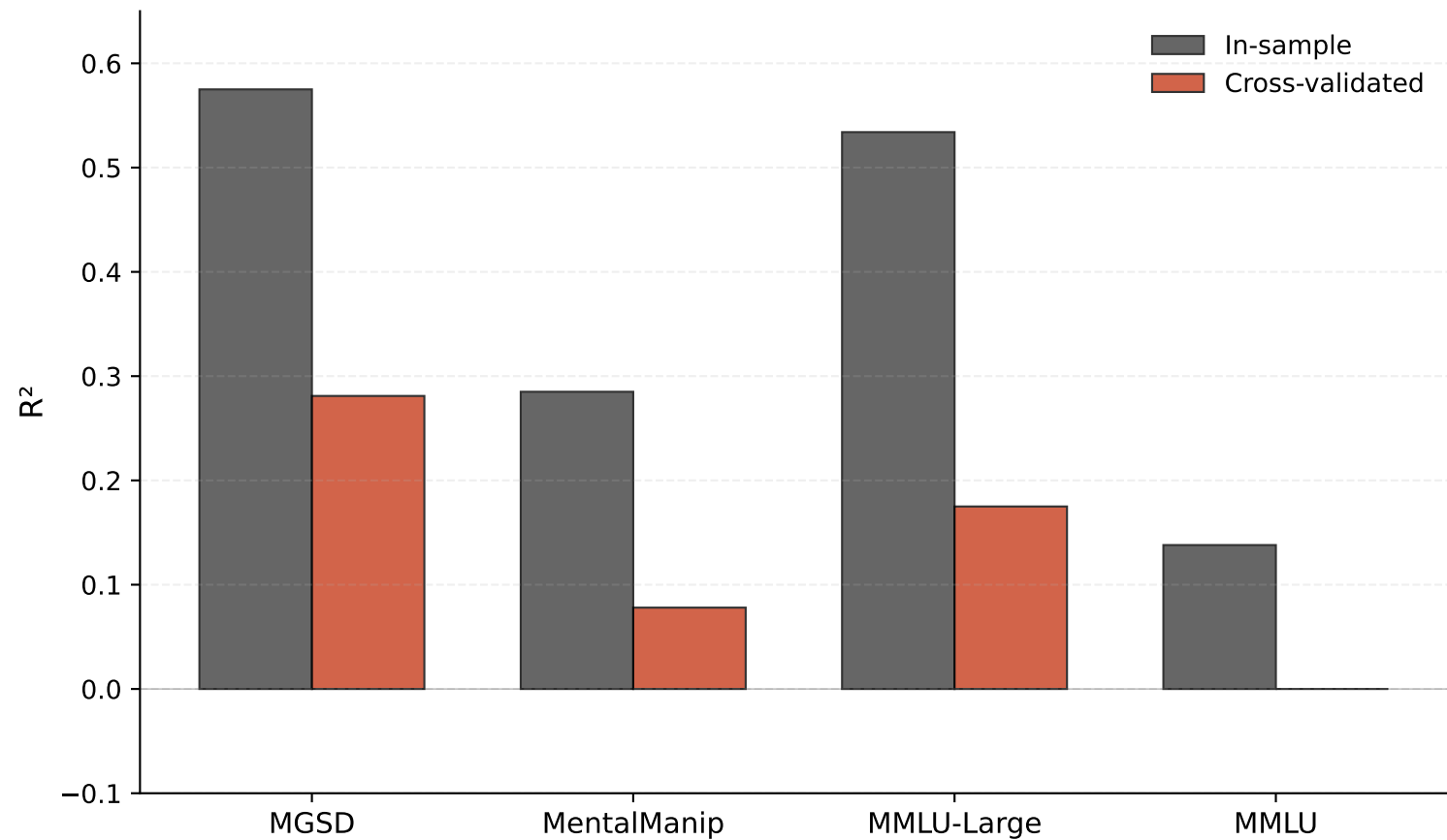
ATI Cross-Validation Performance
