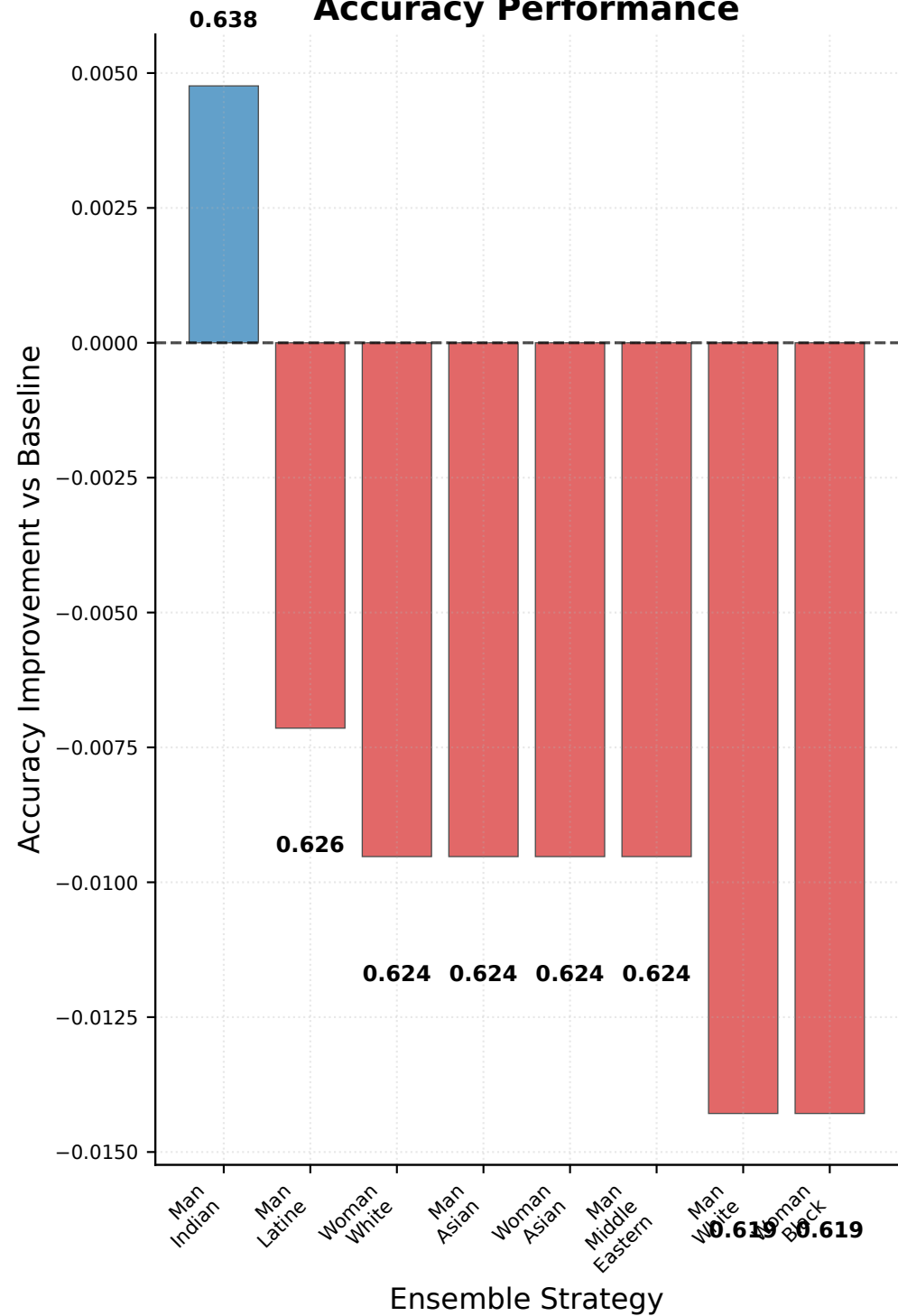
Accuracy Performance
