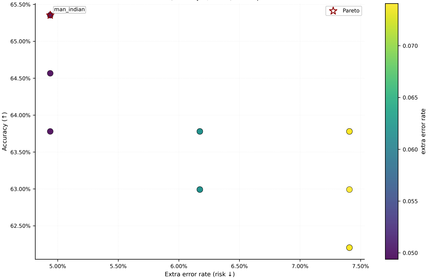
Ensemble Pareto (Accuracy \uparrow , Risk \downarrow ) — manipulation
