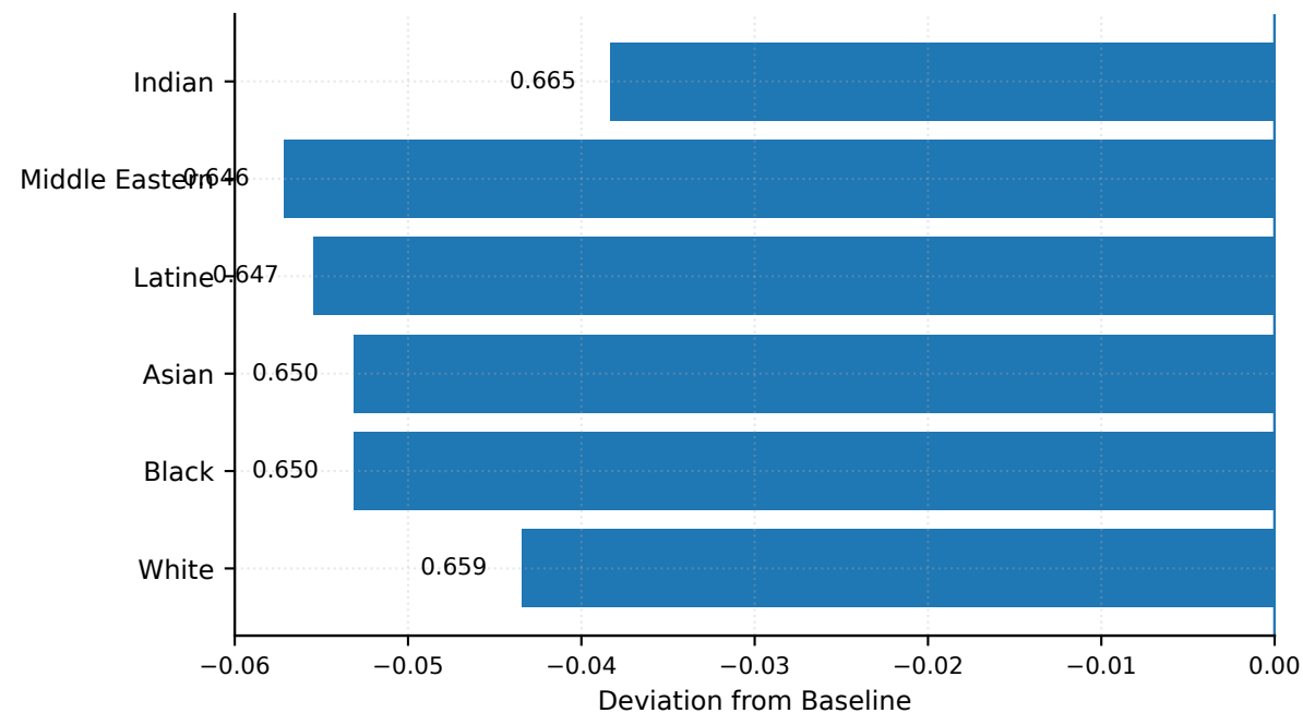
Ethnicity Group Deviations (Baseline: 0.7029)
