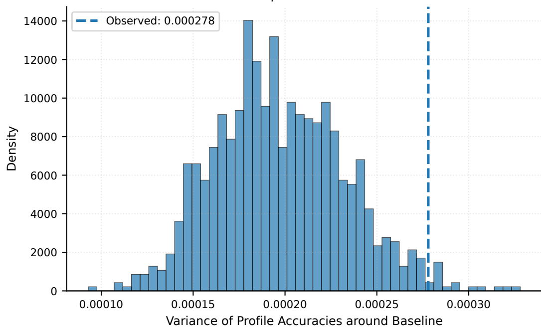
Overall Profile Variance Test p = 0.0160
