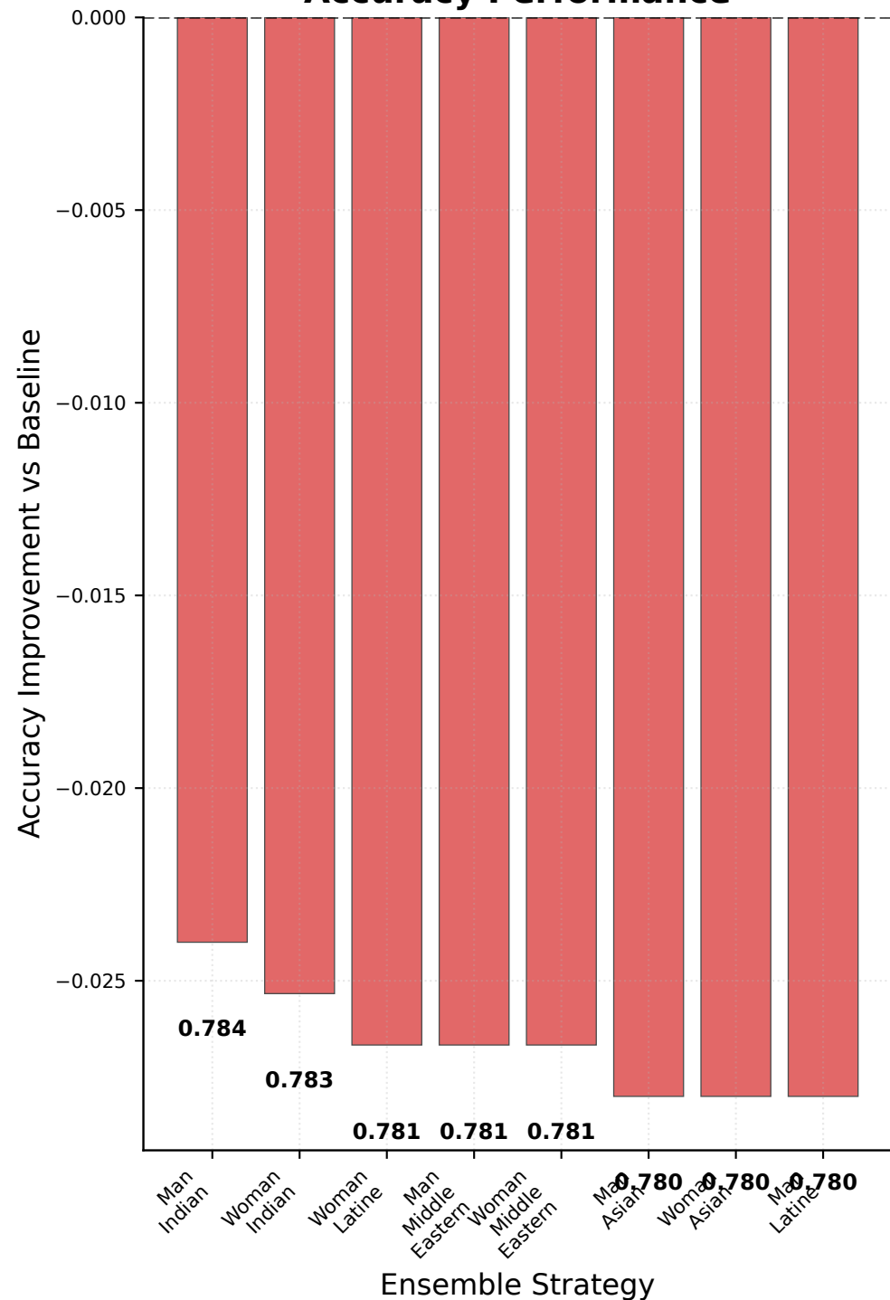
Accuracy Performance
