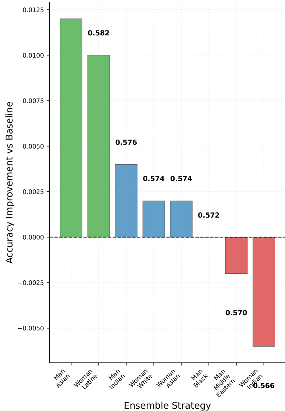
Accuracy Performance
