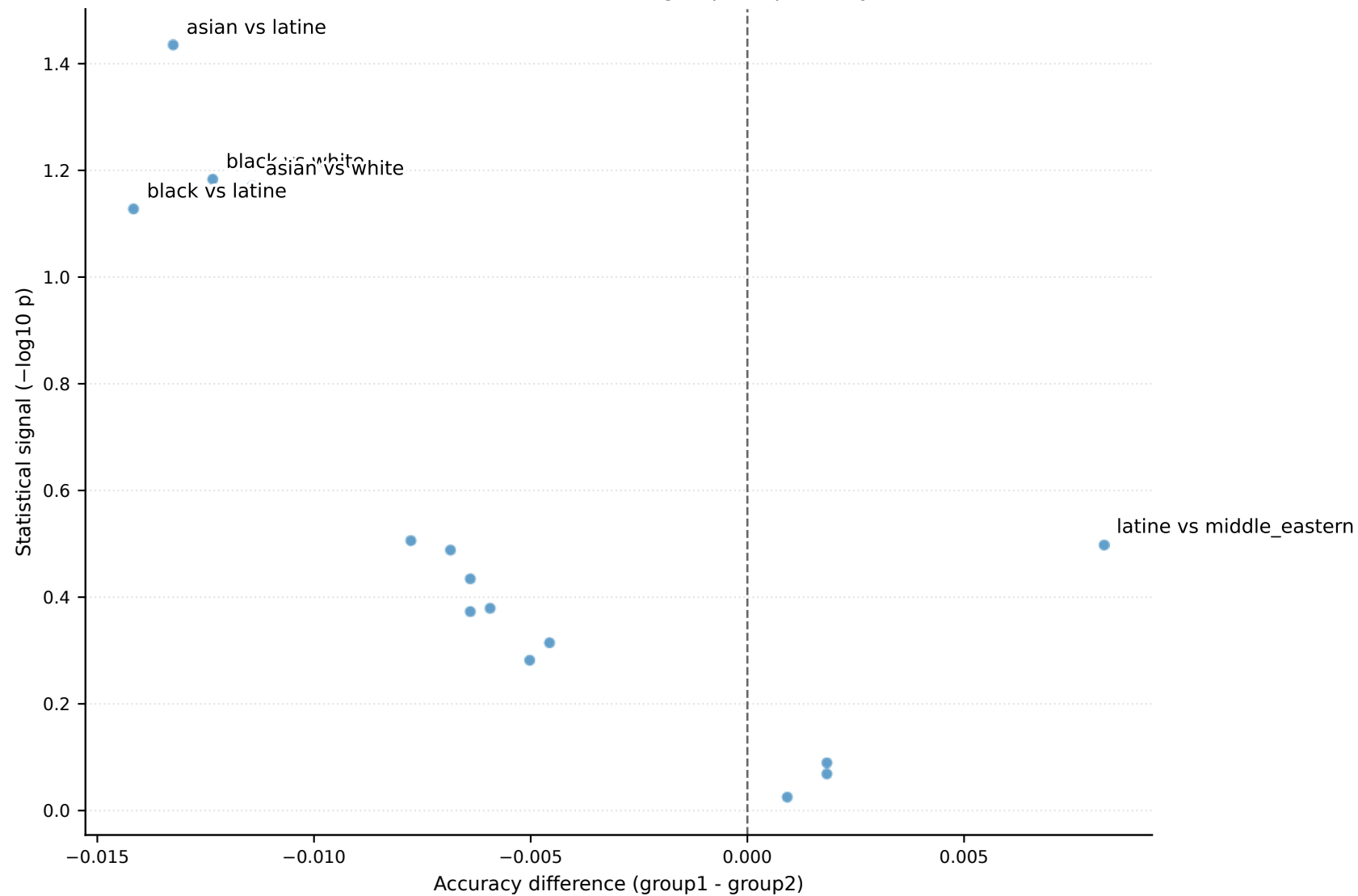
Volcano — Difference vs -\log_{10}(p) (exploratory)
