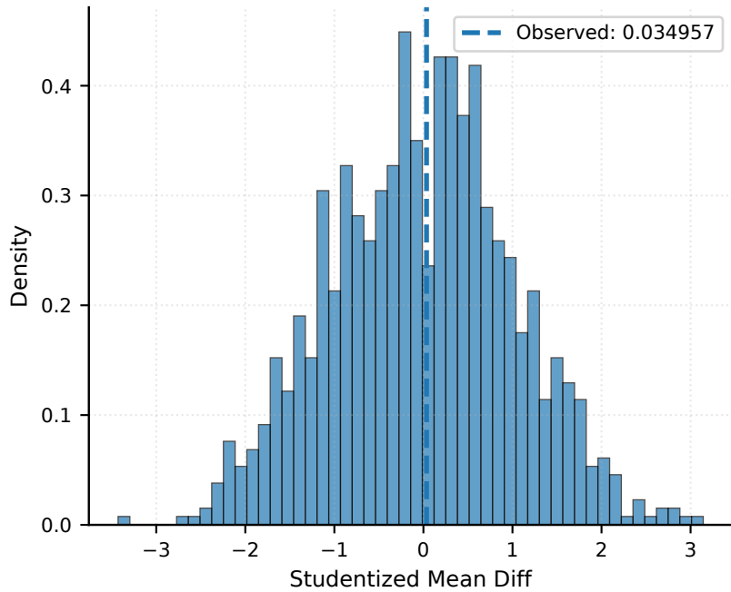
Overall Profile Variance Test p = 0.7153
