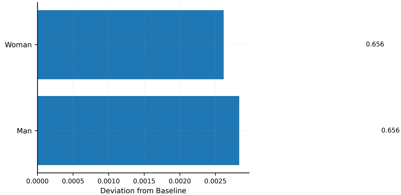
Gender Group Deviations (Baseline: 0.6536)
