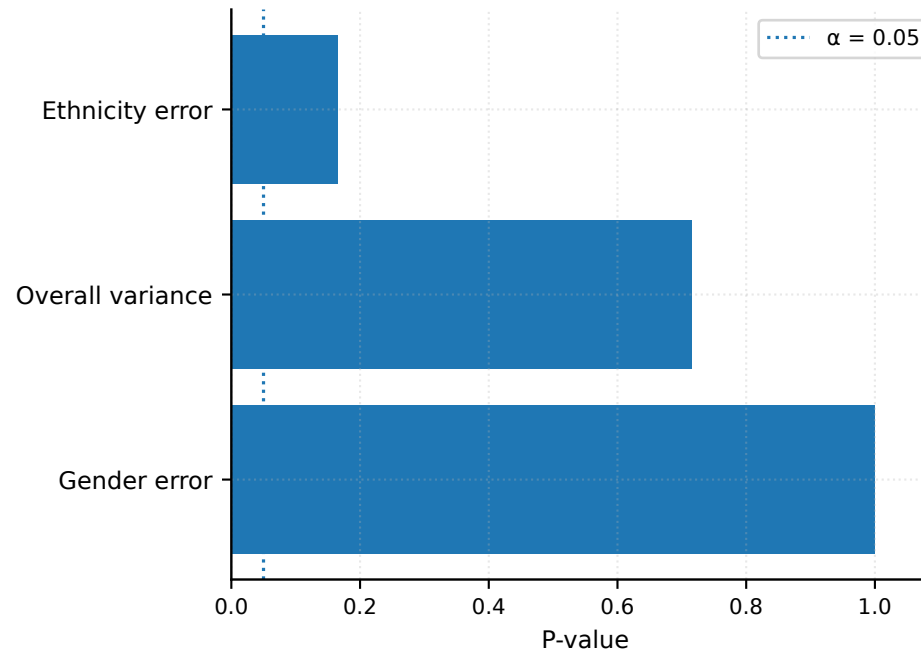
Permutation Test P-values
