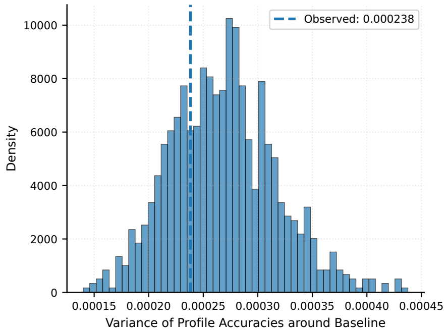
Overall Profile Variance Test p = 0.7153
