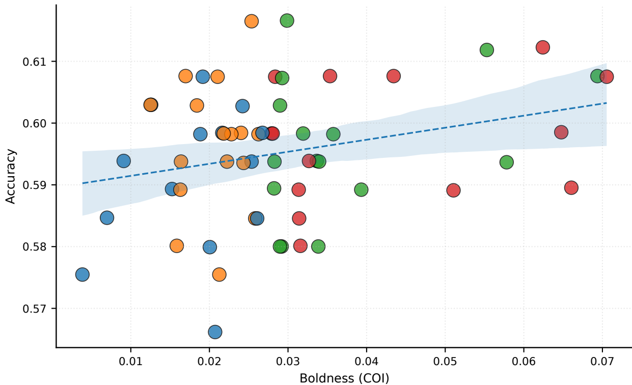
Boldness (COI) vs Accuracy
