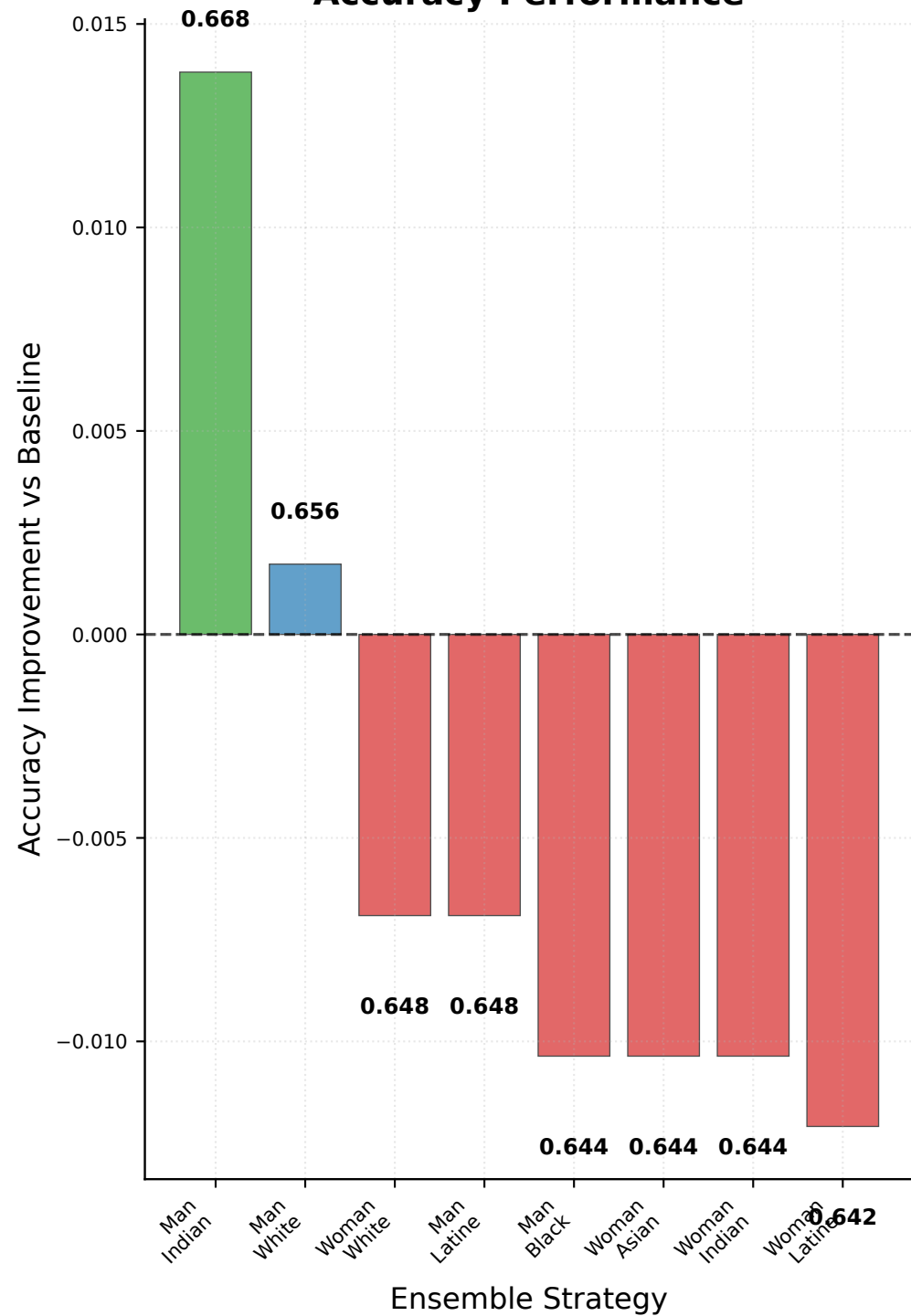
Accuracy Performance
